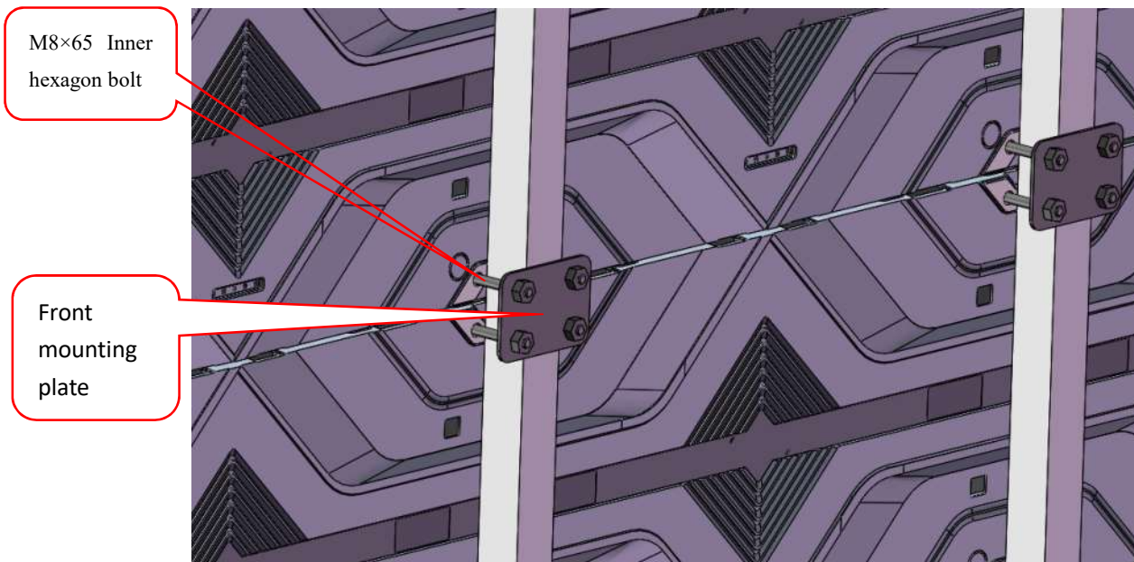
Fig 2-6 Back view of front maintenance Installation Details
