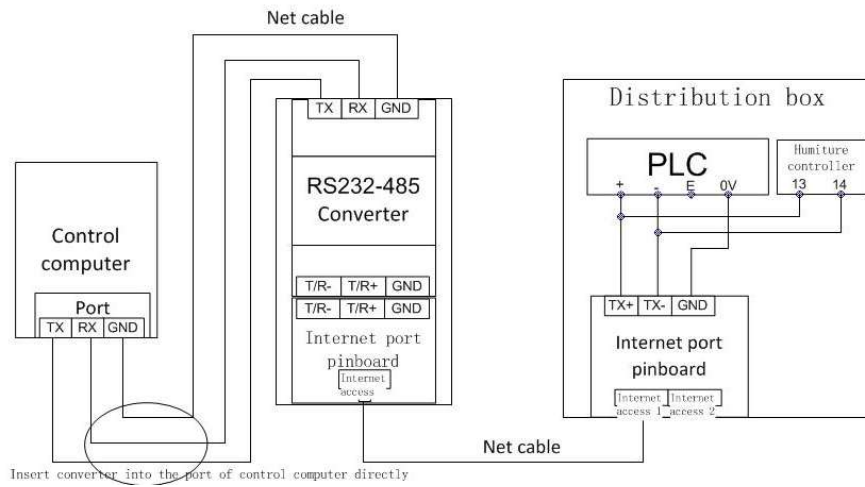
Fig 2-29 Distribution Box PLC Connection Diagram
