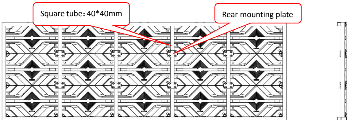
Fig 2-15 Rear View of Cabinet Installation
