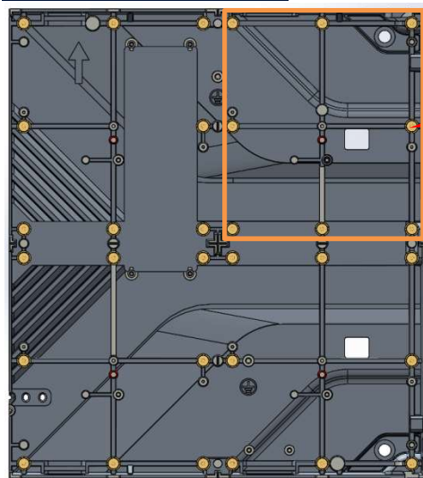
Fig 2-22 Adjustable magnet
