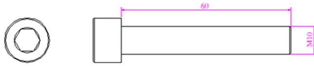
Fig 2-13 Rear installation M10×60 Inner hexagon bolt
