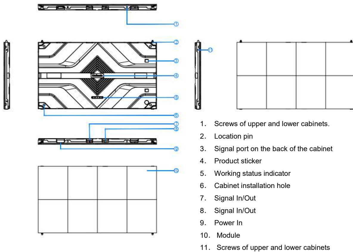
Fig 1-1 Cabinet Appearance
