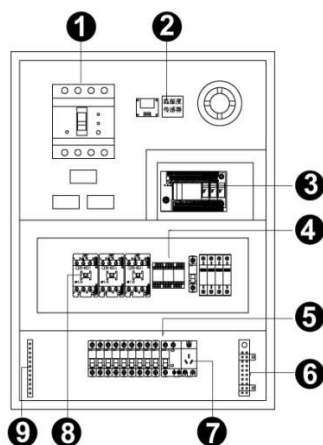
Fig 2-28 Internal Structure of Distribution Box
