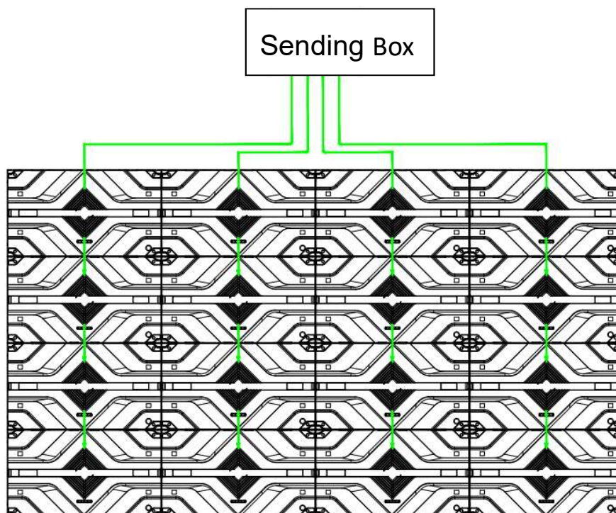
Fig 2-26 Signal Cable Connection Diagram of UMini W1.2
