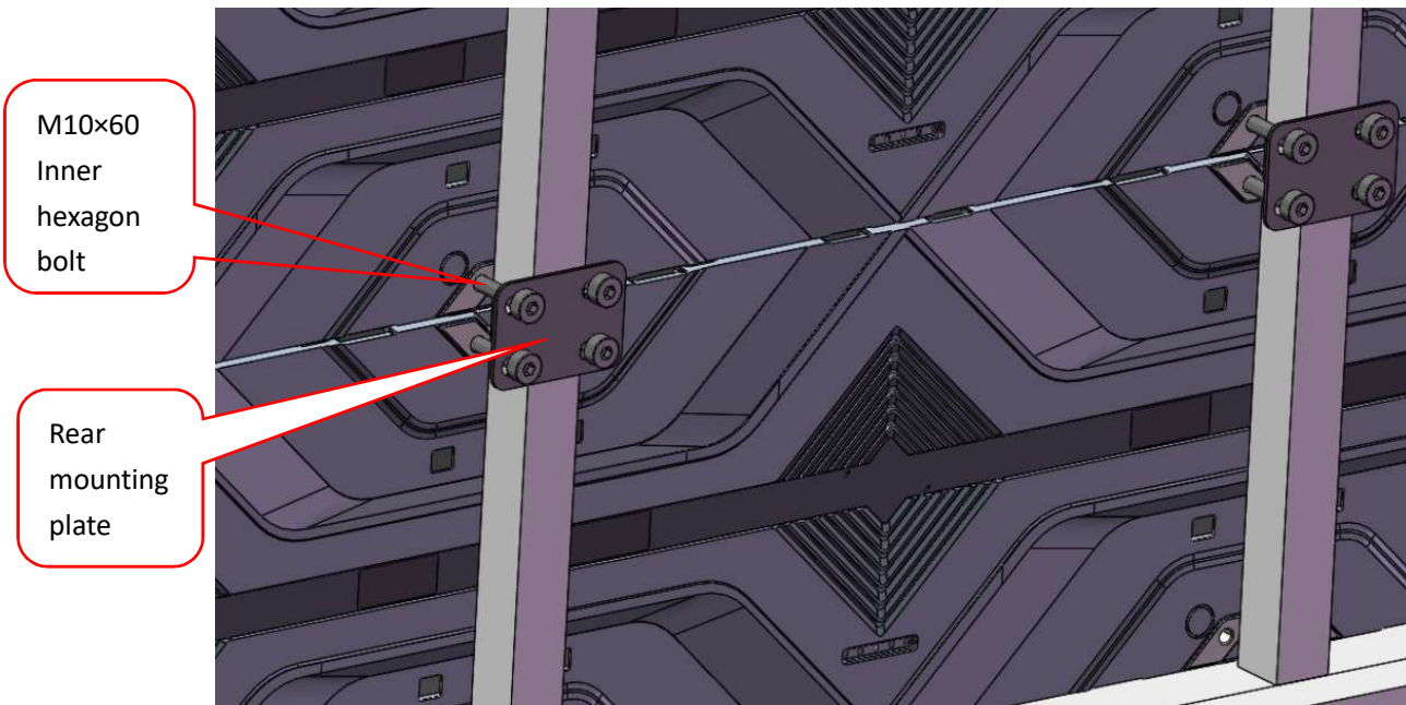
Fig 2-14 Back view of rear maintenance Installation Details
