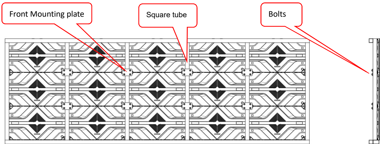
Fig 2-7 Back view of front maintenance Installation
