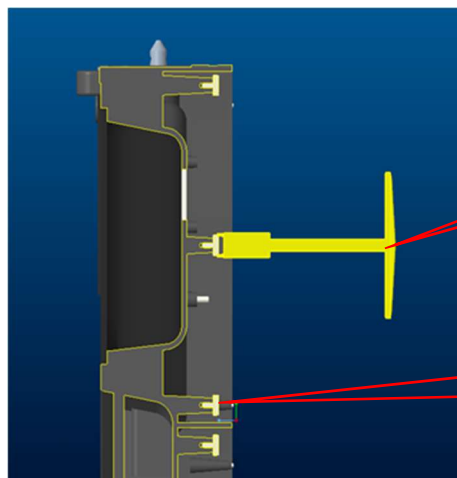
Fig 2-24 Schematic diagram of adjustable magnet
