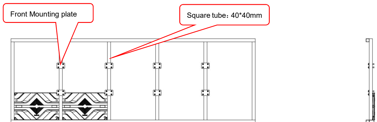
Fig 2-3 Cabinet Fastening
