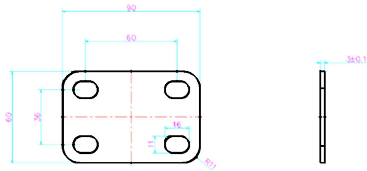
Fig 2-21 Rear Mounting Plate
