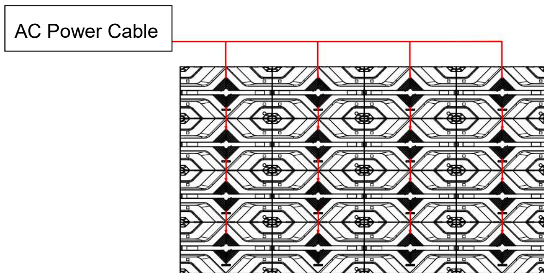
Fig 2-27 Power Cable Connection Diagram of UMini W1.2
