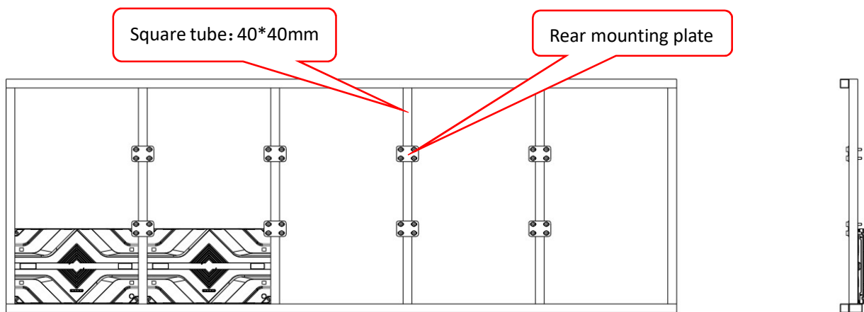
Fig 2-11 Cabinet Fastening
